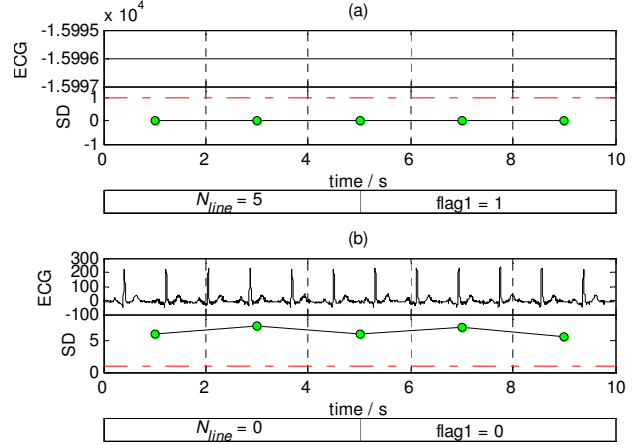
Figure 2. The detections for straight line, (a) ECG with misplaced electrodes, (b) normal ECG.
