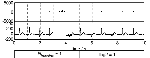
Figure 3. The ECG with huge impulse (upper panel) and ECG removing huge impulse (lower panel).
