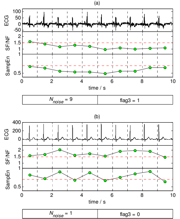
Figure 4. The results of the SF/NF and SampEn for, (a) an ECG with strong Gauss noise, and (b) a normal ECG.
