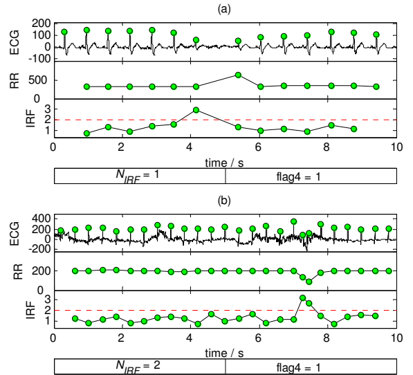
Figure 5. The ECG with huge impulse (upper panel) and ECG removing huge impulse (lower panel).
