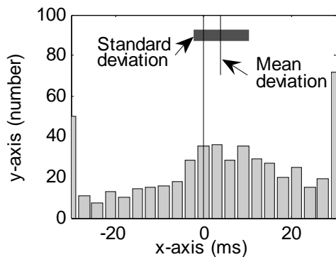
Figure 3. Mean, standard deviations and histogram of differences between the experts' QT markings and the findings of the suggested algorithm.
