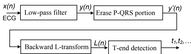
Fig. 1: Diagram of the T-wave end detection algorithm.
